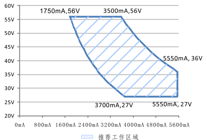
◎ XLG-200-H
